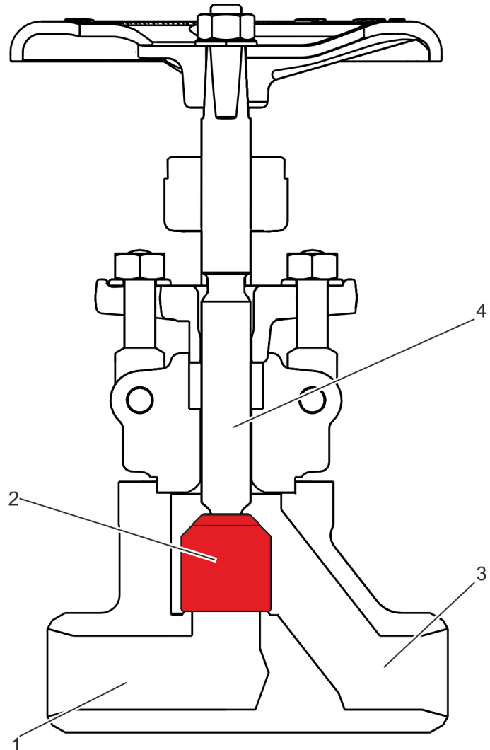
Fig. 8: Sectional view
