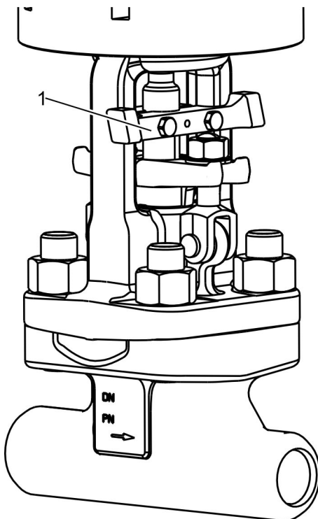
Fig. 5: Mechanical position indicator
