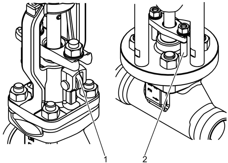
Fig. 11: Packing bolts
